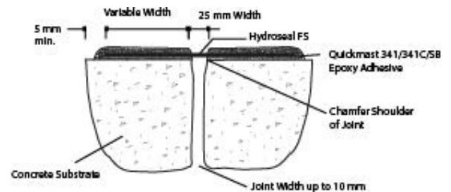
Construction Joints
